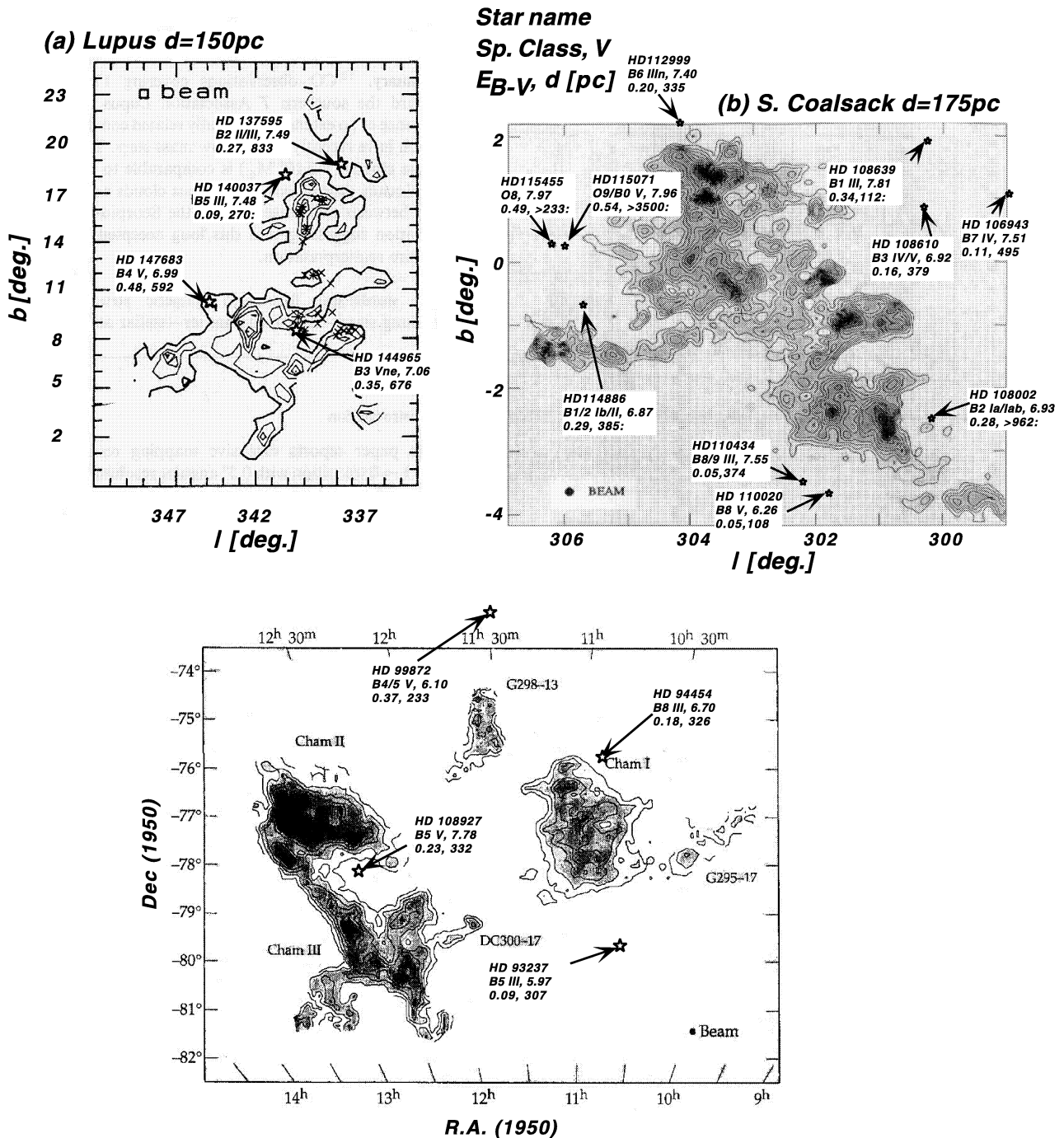
Figure 1. The UHRF target stars are plotted on CO ( J = 1–0) maps. For each star some basic information is listed. Adapted (with permission from Astronomy and Astrophysics) from Murphy et al. (1986) for Lupus, Nyman et al. (1989) for the Southern Coalsack and Boulanger et al. (1998) for Chamaeleon.
